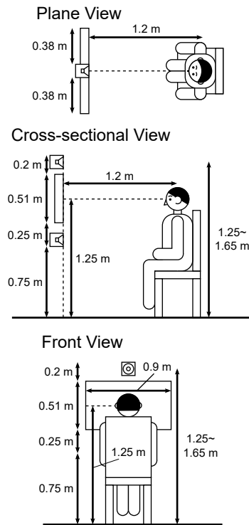
Fig. 1 Position of viewers, display and the loudspeakers in the audio-visual experiment.
